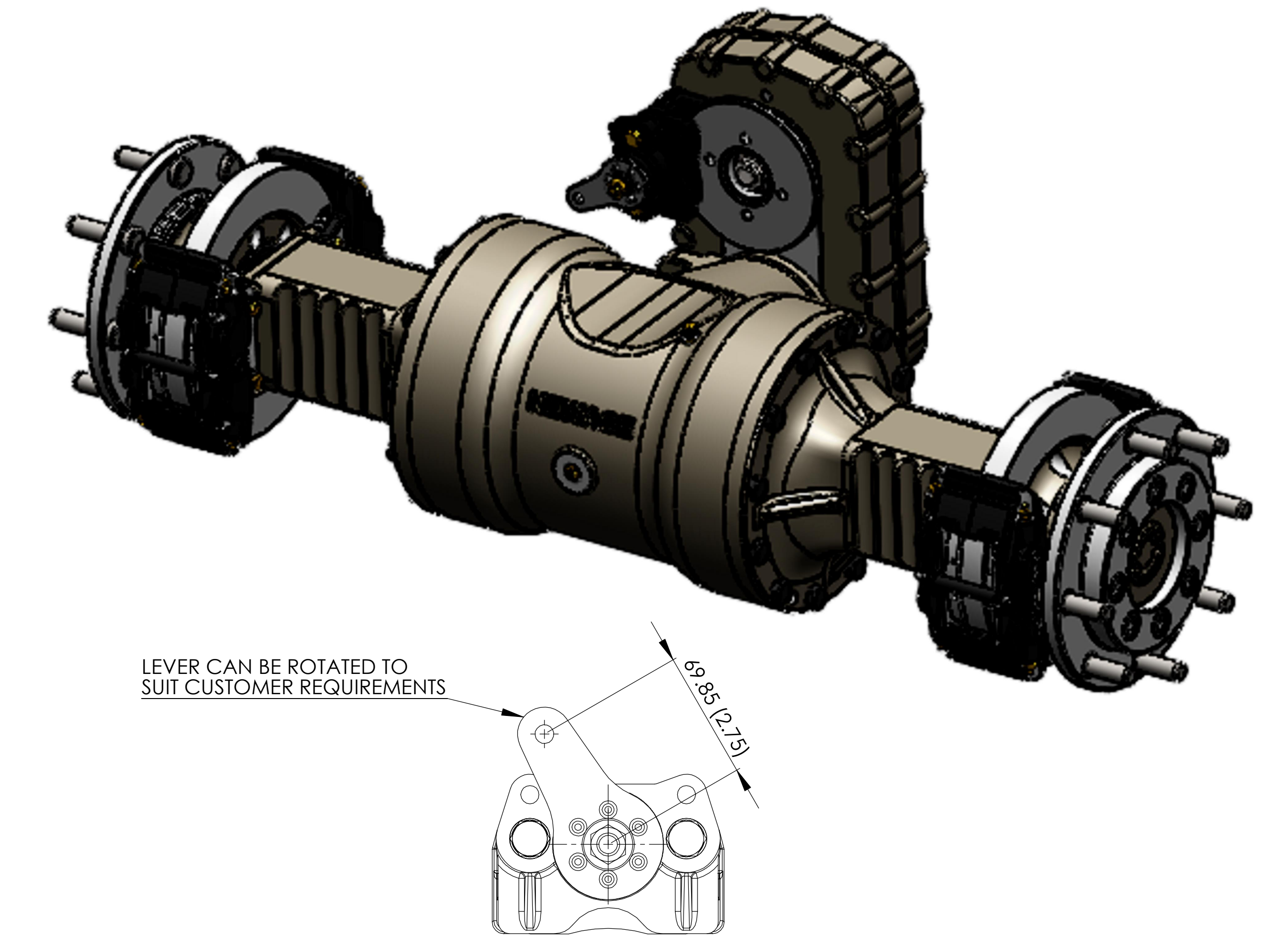
PARK BRAKE DETAIL VIEW SCALE 1:2
